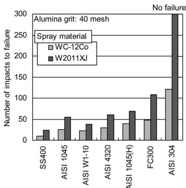
Fig. 4 Influence of substrate material on the impact resistance of WC-12Co and W2011XJ coatings
